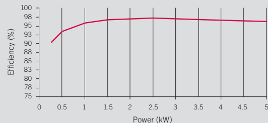
Efficiency INGECON® SUN 5TL M V dc = 680 V
