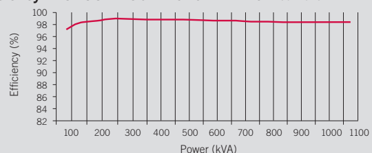
Efficiency INGECON® SUN 1070TL X420 V dc = 625 V
